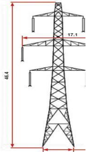
L8c D STD 400kV SUSPENSION LATTICE PYLON
